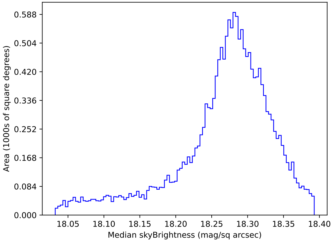
roll_uniform_early_half_mjdp0_v3.4_10yrs WFD y band: Median skyBrightness
