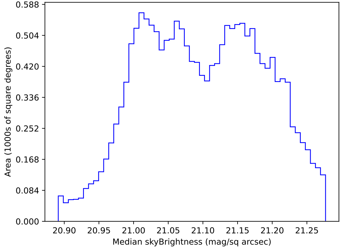
roll_uniform_early_half_mjdp0_v3.4_10yrs WFD r band: Median skyBrightness
