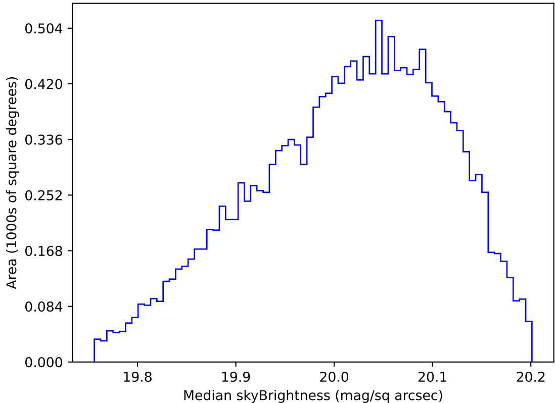
roll_uniform_early_half_mjdp0_v3.4_10yrs WFD i band: Median skyBrightness
