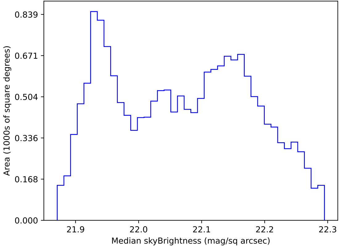
roll_uniform_early_half_mjdp0_v3.4_10yrs WFD g band: Median skyBrightness
