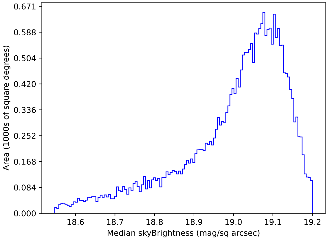
roll_uniform_early_half_mjdp0_v3.4_10yrs All sky z band: Median skyBrightness
