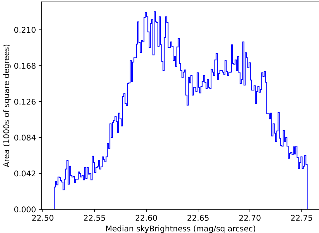
roll_uniform_early_half_mjdp0_v3.4_10yrs All sky u band: Median skyBrightness
