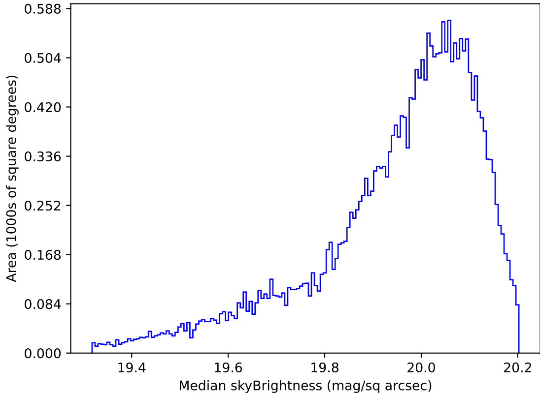
roll_uniform_early_half_mjdp0_v3.4_10yrs All sky i band: Median skyBrightness
