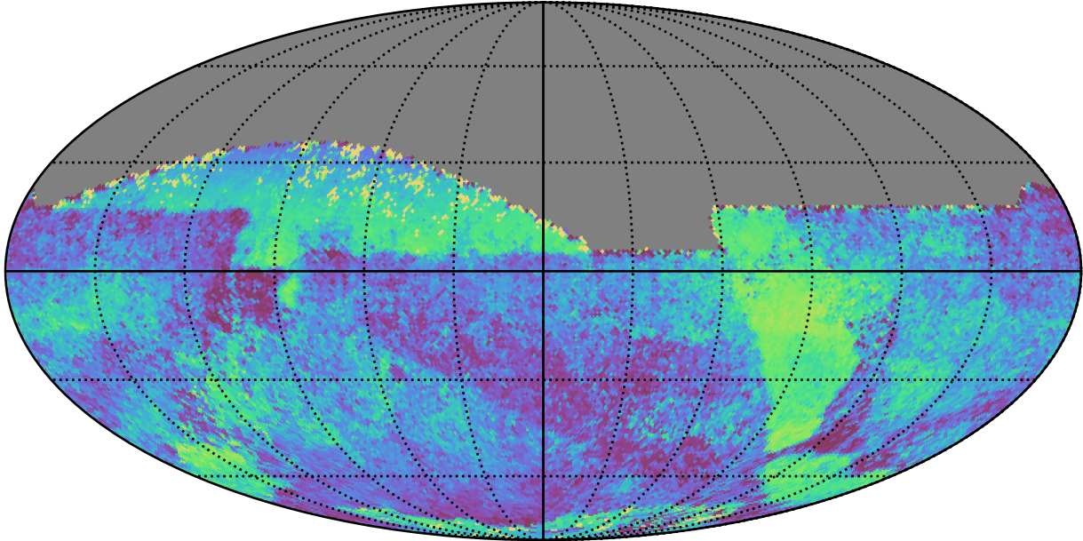
roll_uniform_early_half_mjdp0_v3.4_10yrs All sky all bands: Median skyBrightness
