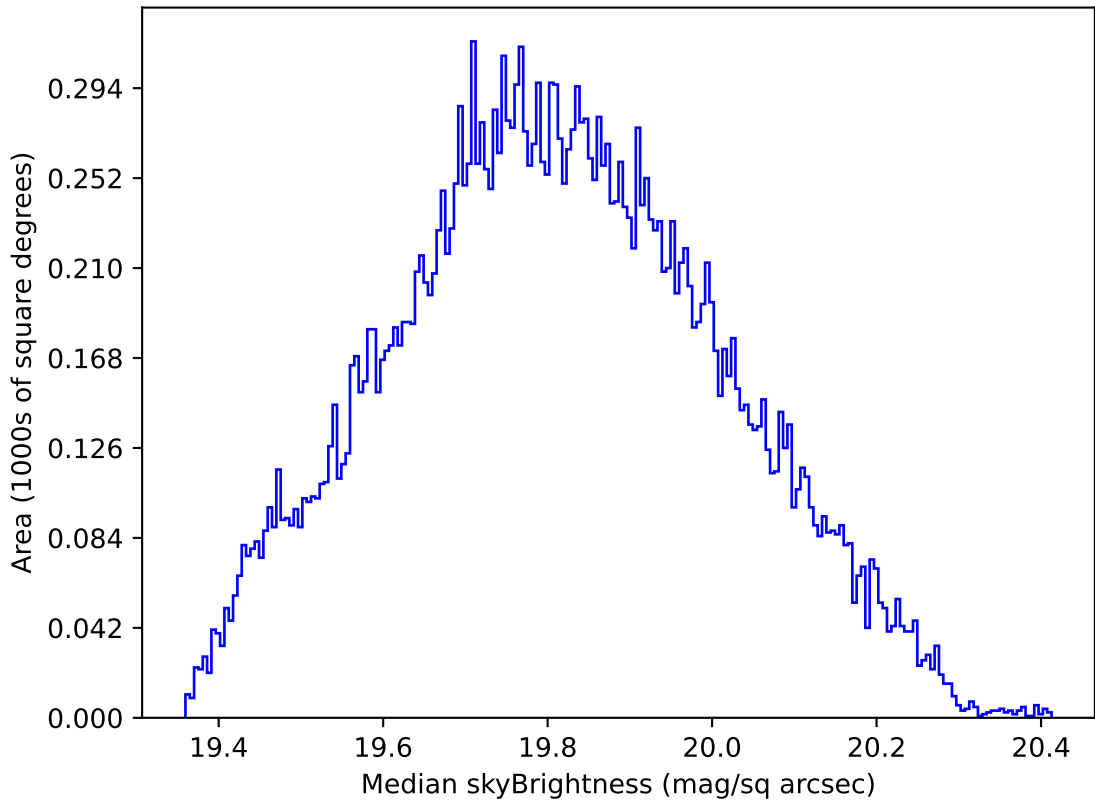
roll_uniform_early_half_mjdp0_v3.4_10yrs All sky all bands: Median skyBrightness
