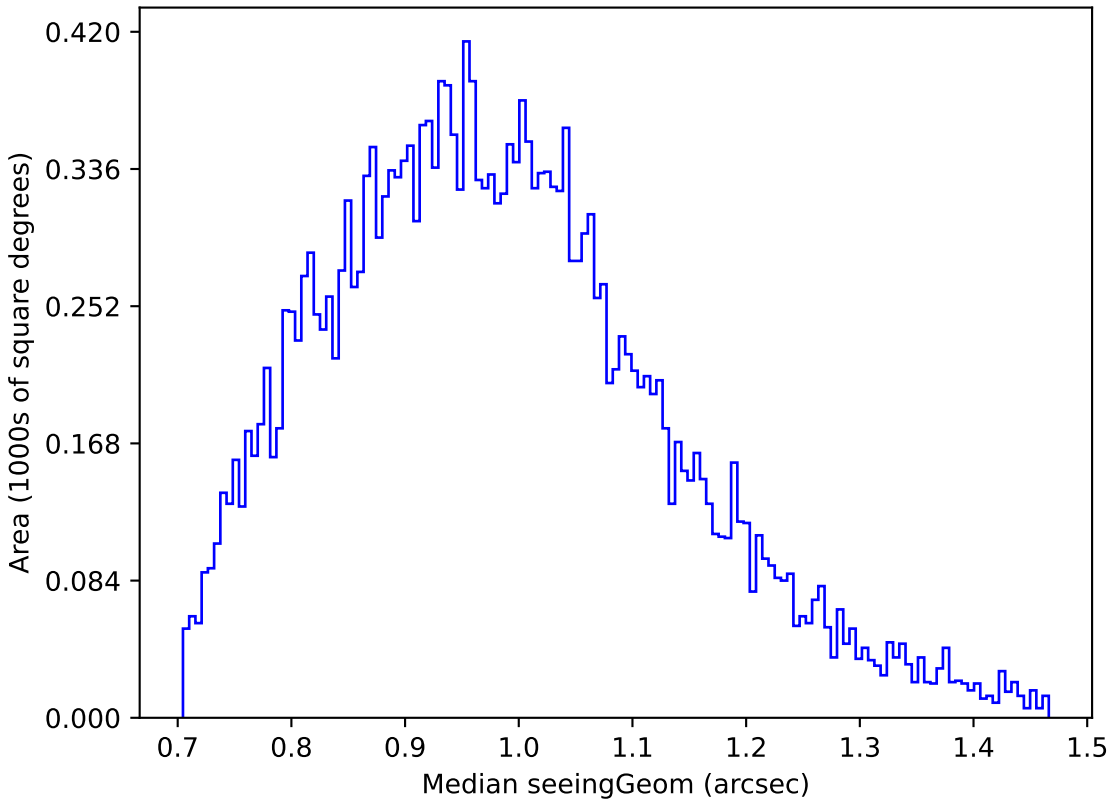
roll_uniform_early_half_mjdp0_v3.4_10yrs Yr 1 u band: Median seeingGeom
