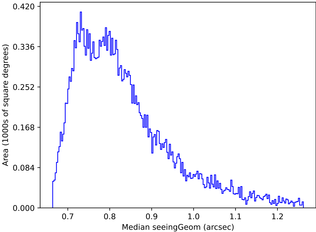
roll_uniform_early_half_mjdp0_v3.4_10yrs Yr 1 i band: Median seeingGeom
