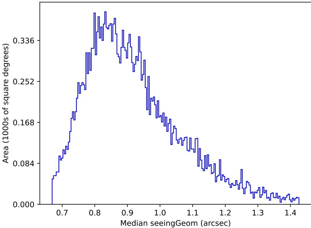
roll_uniform_early_half_mjdp0_v3.4_10yrs Yr 1 g band: Median seeingGeom
