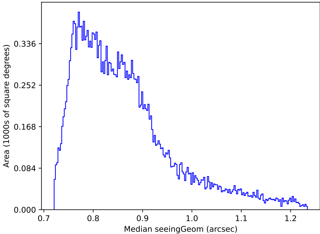
roll_uniform_early_half_mjdp0_v3.4_10yrs Yr 1 all bands: Median seeingGeom
