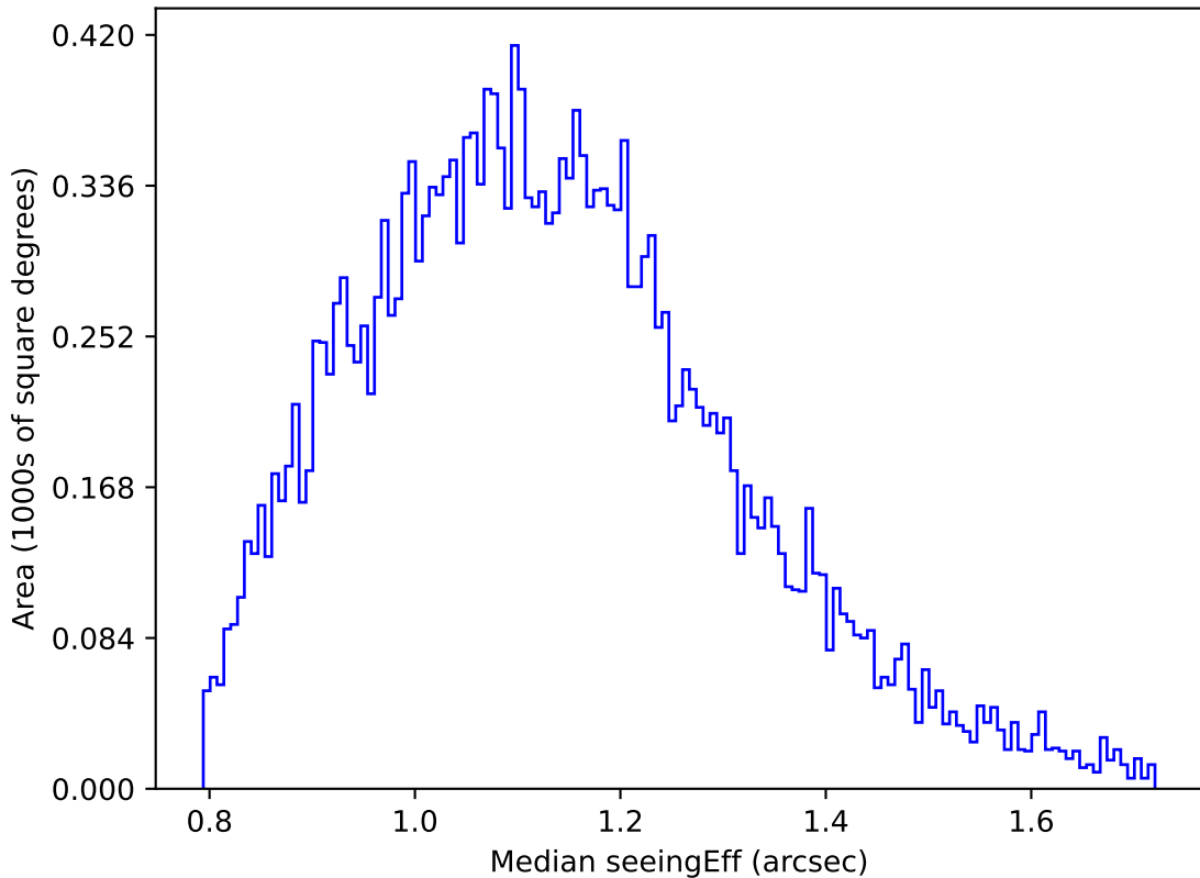
roll_uniform_early_half_mjdp0_v3.4_10yrs Yr 1 u band: Median seeingEff
