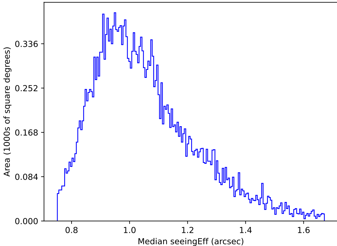
roll_uniform_early_half_mjdp0_v3.4_10yrs Yr 1 g band: Median seeingEff
