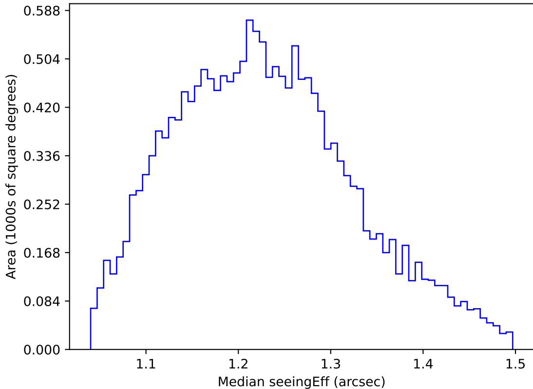
roll_uniform_early_half_mjdp0_v3.4_10yrs WFD u band: Median seeingEff
