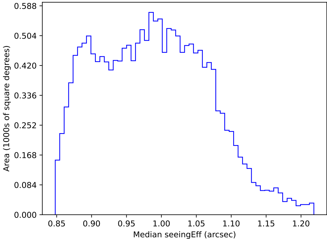
roll_uniform_early_half_mjdp0_v3.4_10yrs WFD i band: Median seeingEff
