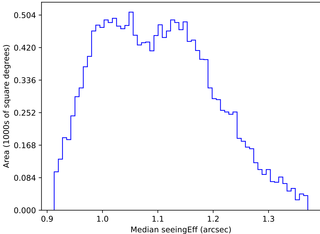
roll_uniform_early_half_mjdp0_v3.4_10yrs WFD g band: Median seeingEff
