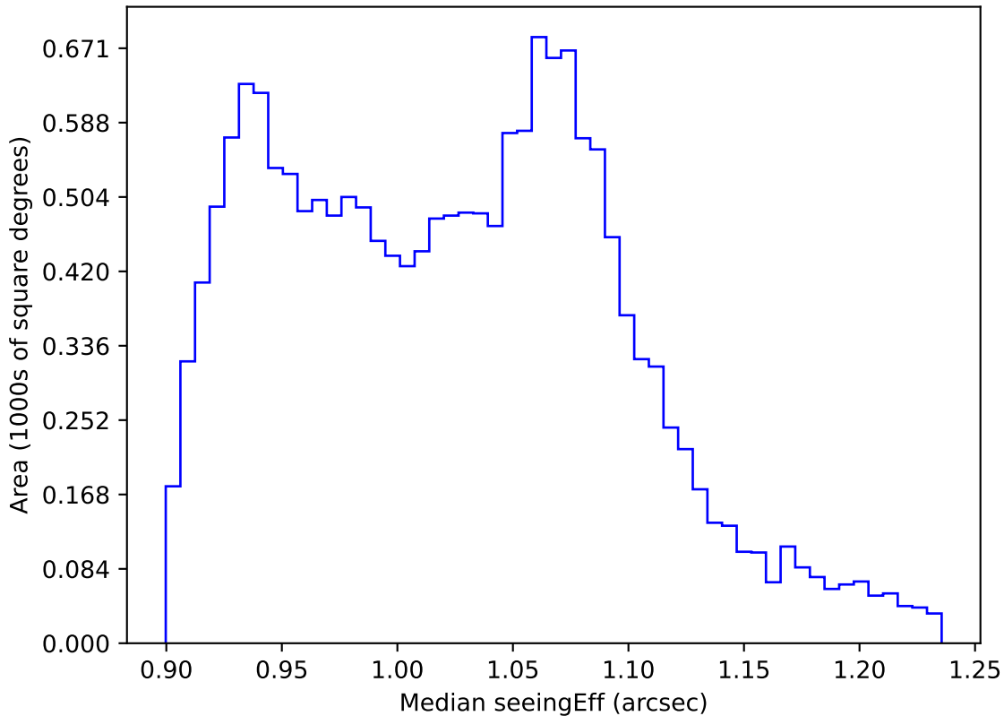
roll_uniform_early_half_mjdp0_v3.4_10yrs WFD all bands: Median seeingEff
