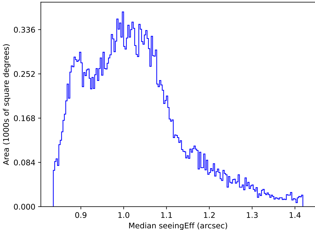
roll_uniform_early_half_mjdp0_v3.4_10yrs All sky i band: Median seeingEff
