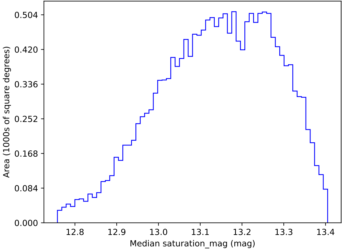
roll_uniform_early_half_mjdp0_v3.4_10yrs WFD y band: Median saturation_mag
