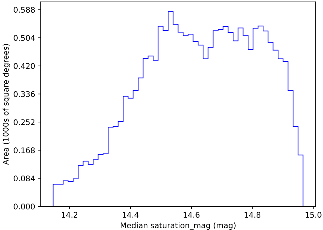
roll_uniform_early_half_mjdp0_v3.4_10yrs WFD r band: Median saturation_mag
