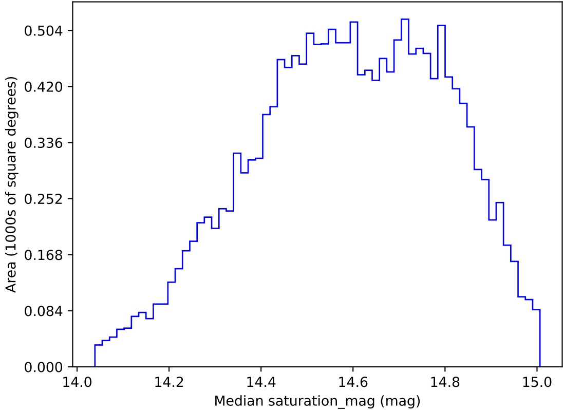
roll_uniform_early_half_mjdp0_v3.4_10yrs WFD g band: Median saturation_mag
