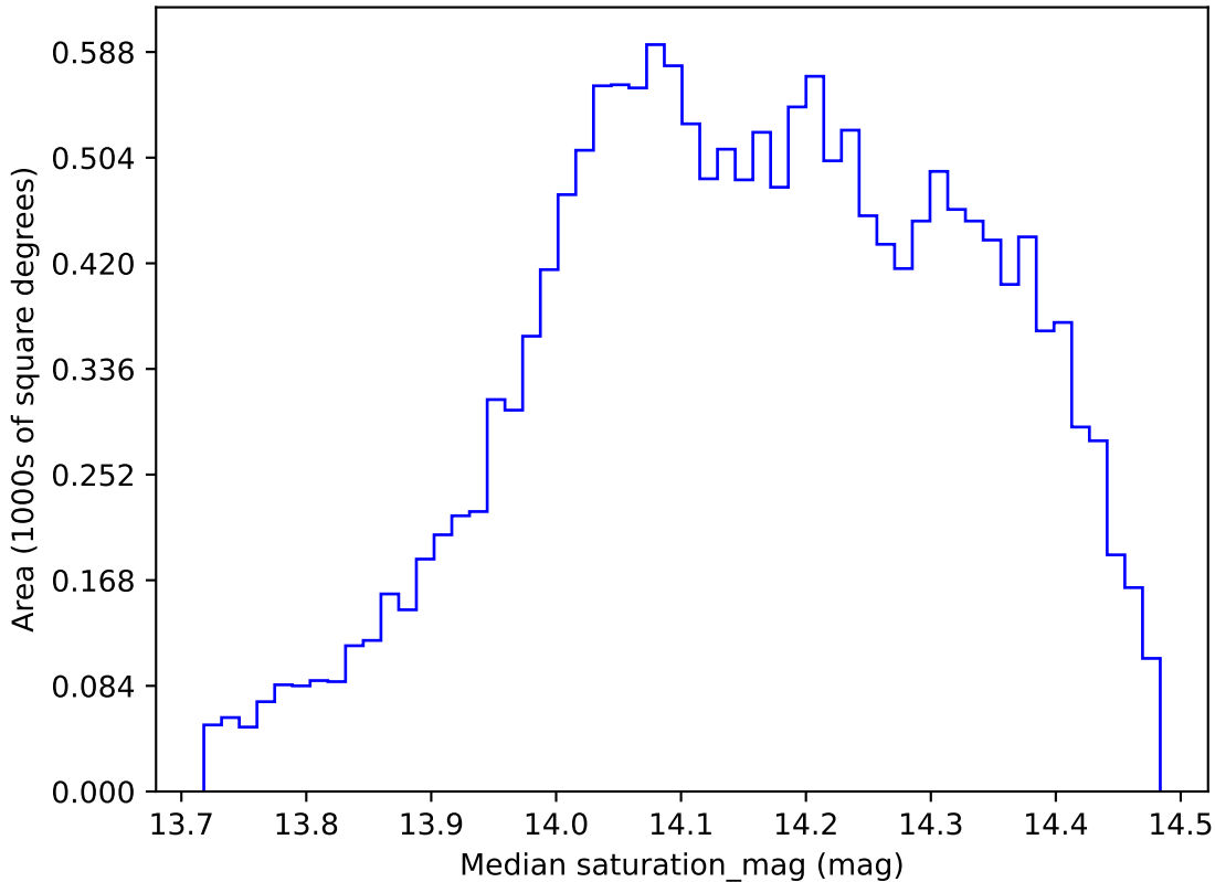
roll_uniform_early_half_mjdp0_v3.4_10yrs WFD all bands: Median saturation_mag
