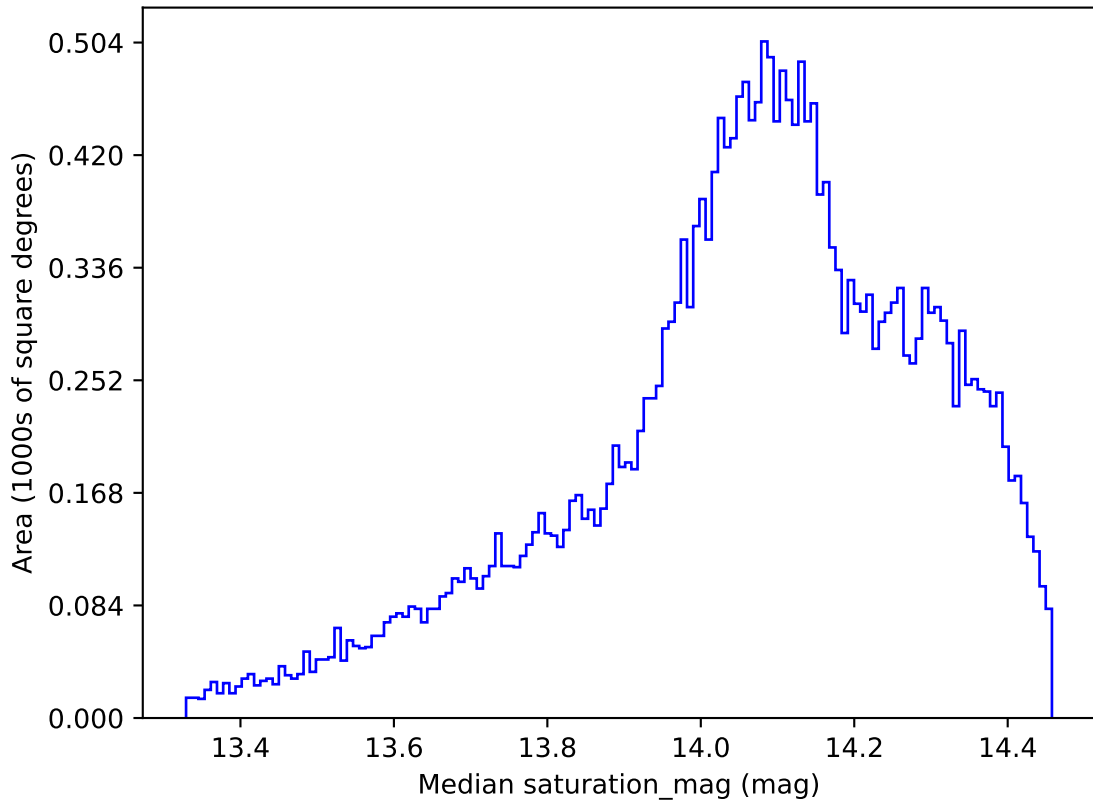
roll_uniform_early_half_mjdp0_v3.4_10yrs All sky z band: Median saturation_mag
