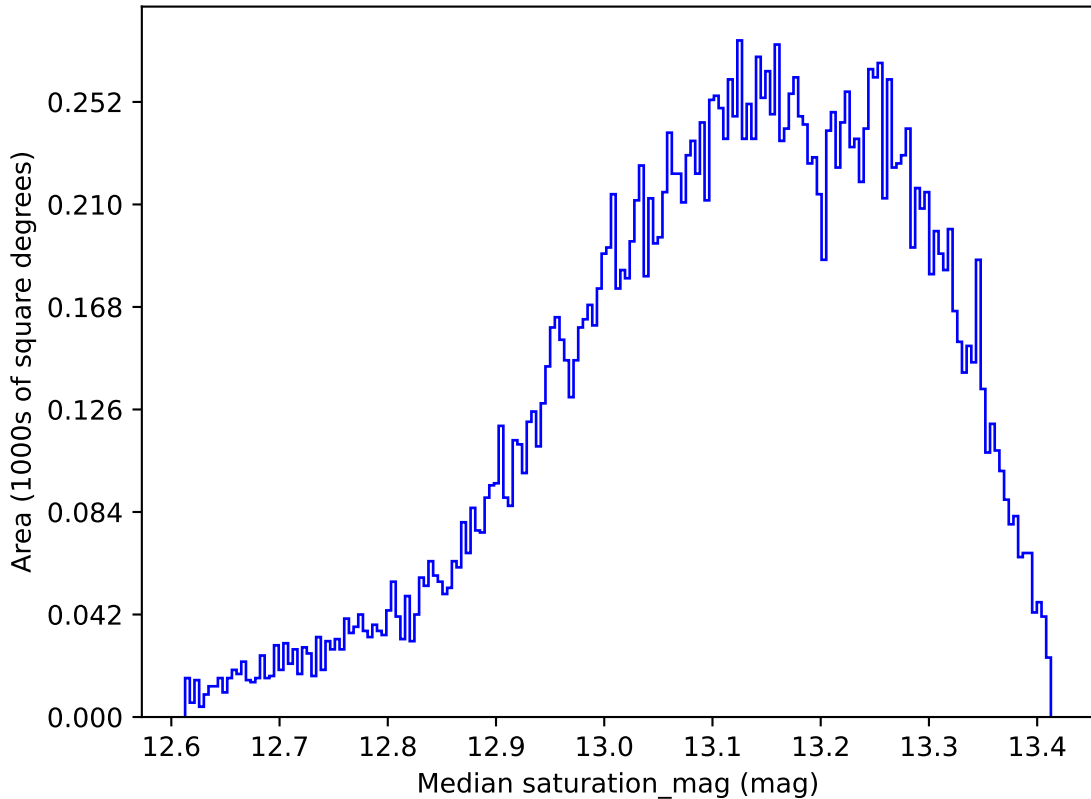
roll_uniform_early_half_mjdp0_v3.4_10yrs All sky y band: Median saturation_mag
