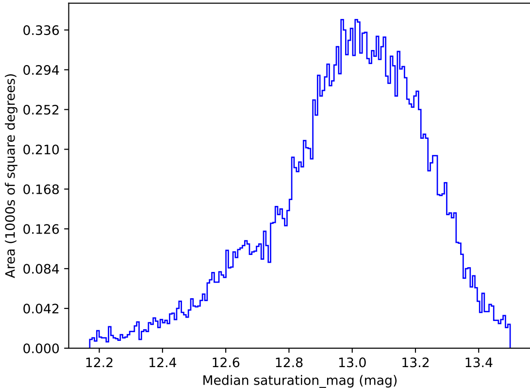
roll_uniform_early_half_mjdp0_v3.4_10yrs All sky u band: Median saturation_mag
