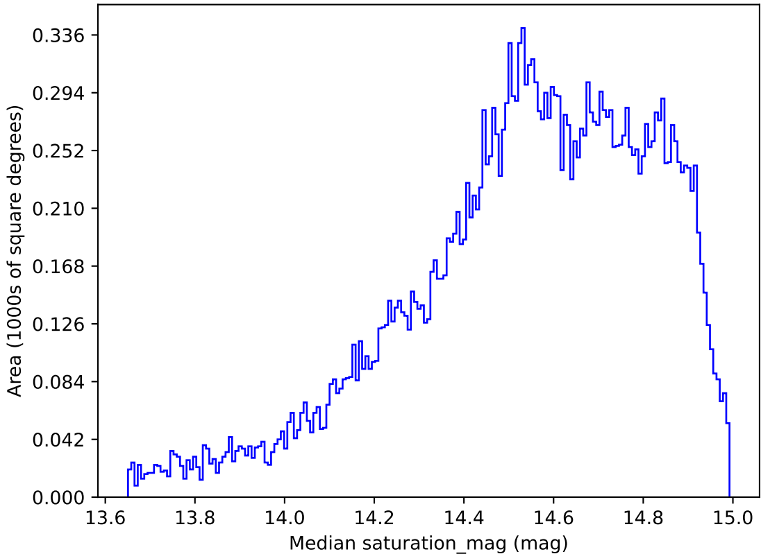
roll_uniform_early_half_mjdp0_v3.4_10yrs All sky r band: Median saturation_mag
