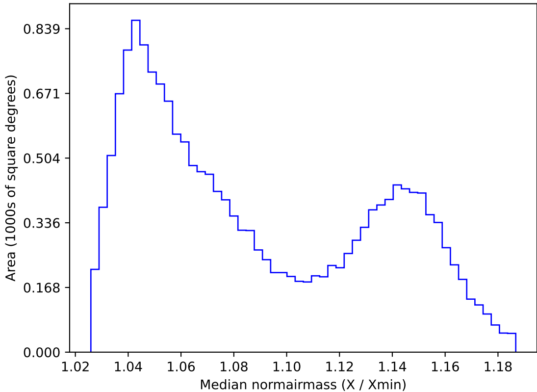
roll_uniform_early_half_mjdp0_v3.4_10yrs WFD y band: Median normairmass
