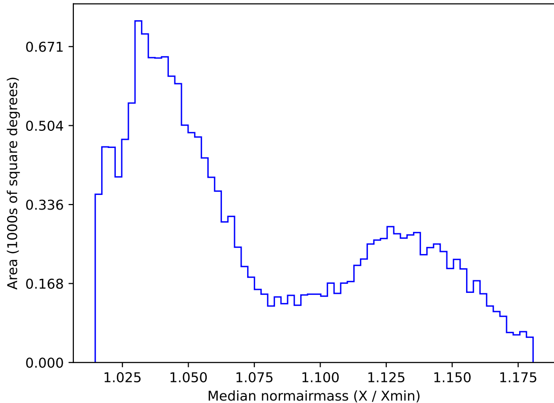
roll_uniform_early_half_mjdp0_v3.4_10yrs WFD r band: Median normairmass
