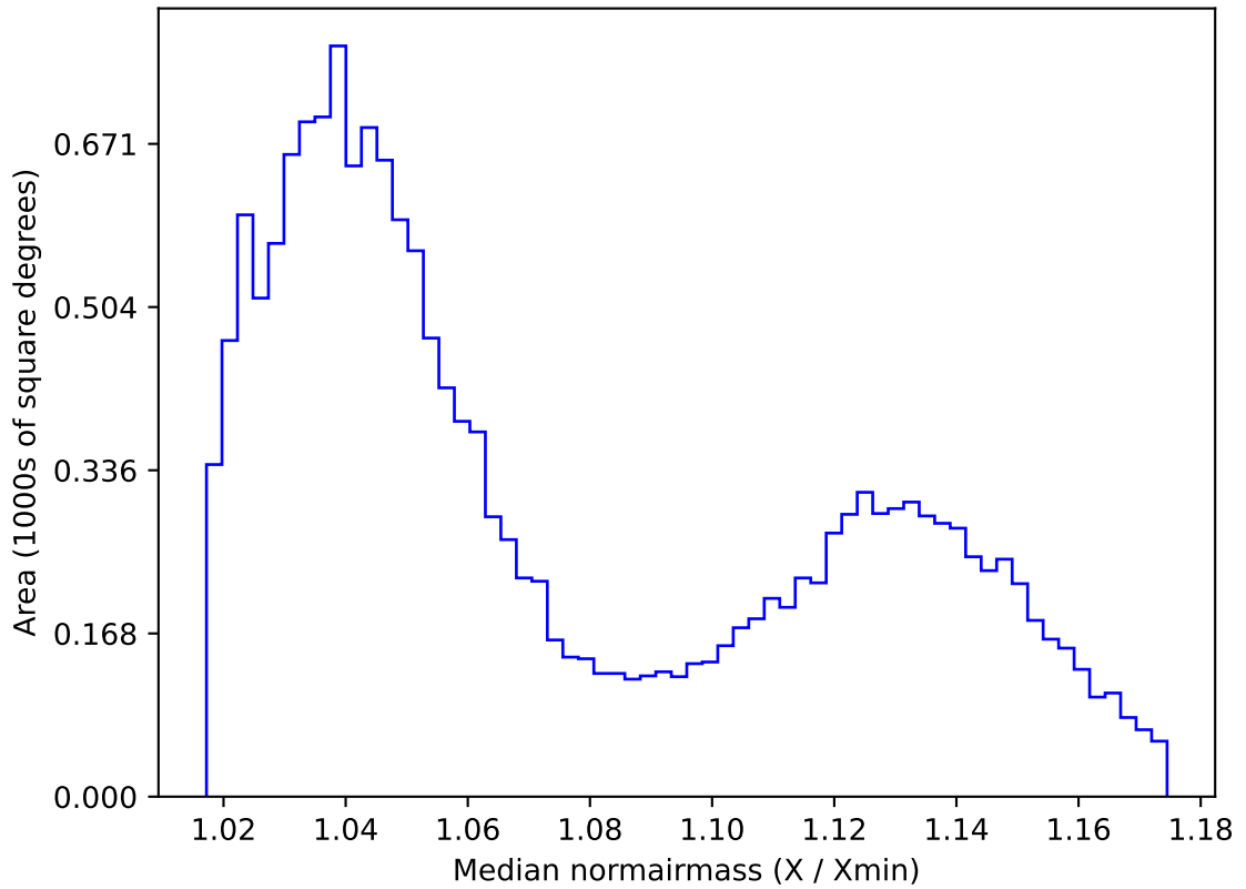
roll_uniform_early_half_mjdp0_v3.4_10yrs WFD i band: Median normairmass
