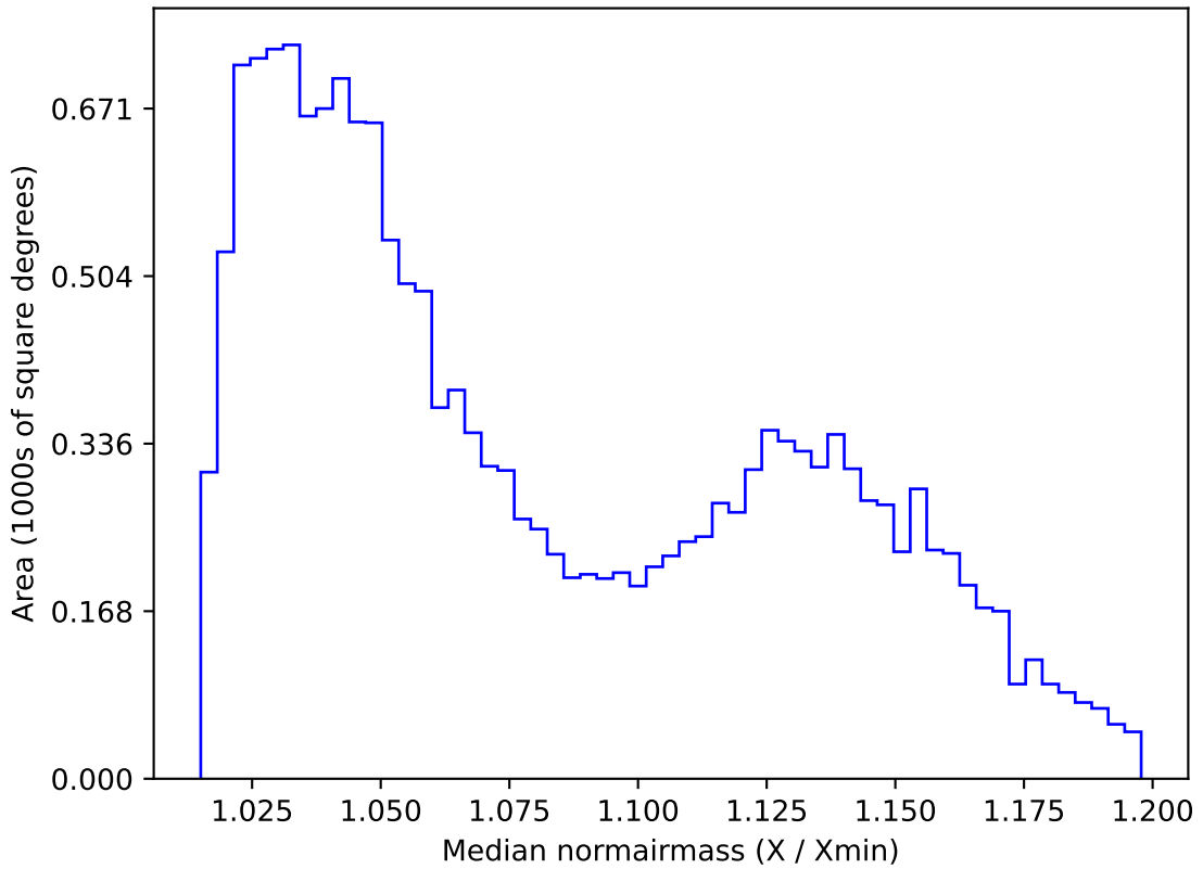
roll_uniform_early_half_mjdp0_v3.4_10yrs WFD g band: Median normairmass
