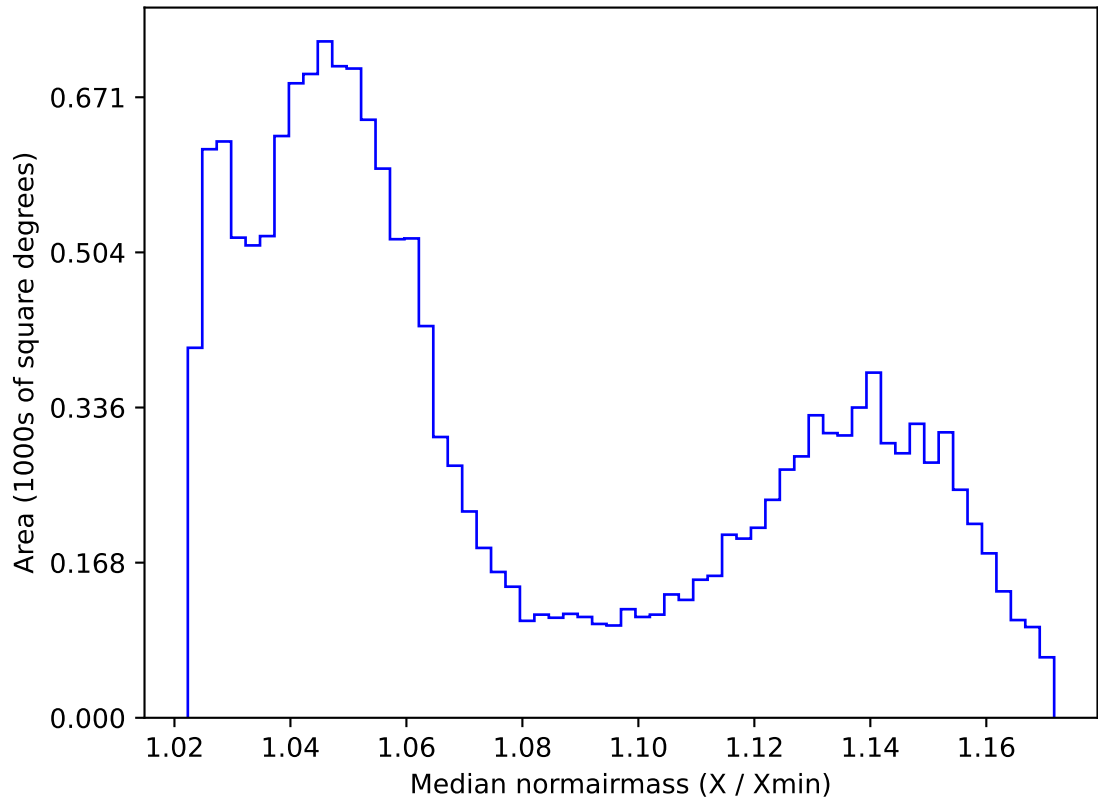
roll_uniform_early_half_mjdp0_v3.4_10yrs WFD all bands: Median normairmass
