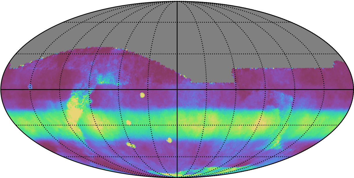
roll_uniform_early_half_mjdp0_v3.4_10yrs All sky all bands: Median normairmass
