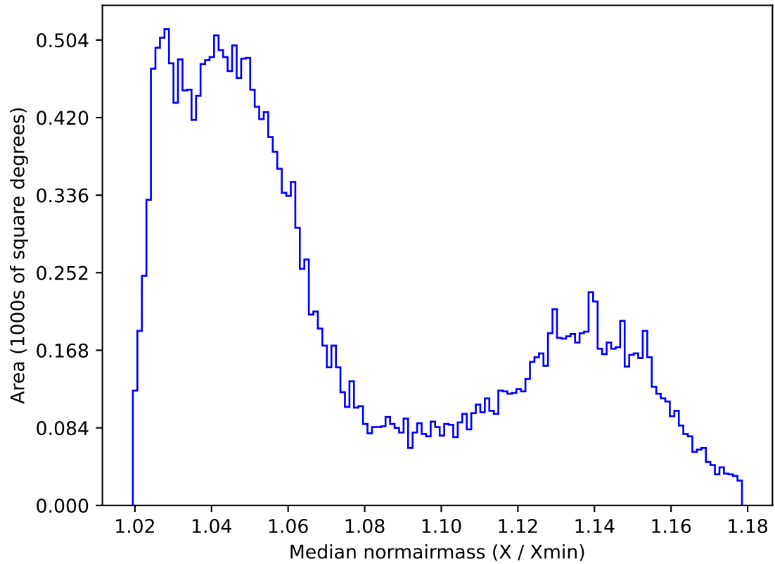
roll_uniform_early_half_mjdp0_v3.4_10yrs All sky all bands: Median normairmass
