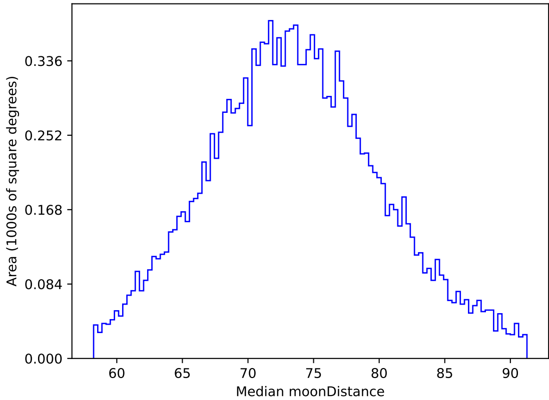
roll_uniform_early_half_mjdp0_v3.4_10yrs WFD z band: Median moonDistance
