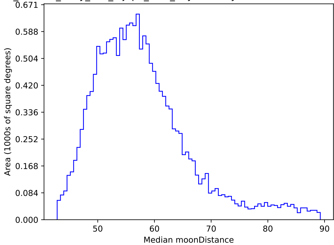
roll_uniform_early_half_mjdp0_v3.4_10yrs WFD y band: Median moonDistance
