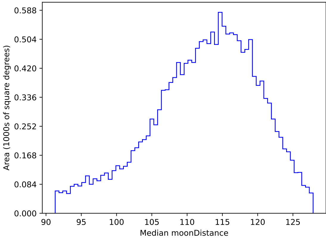
roll_uniform_early_half_mjdp0_v3.4_10yrs WFD r band: Median moonDistance
