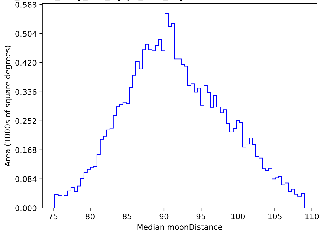
roll_uniform_early_half_mjdp0_v3.4_10yrs WFD i band: Median moonDistance
