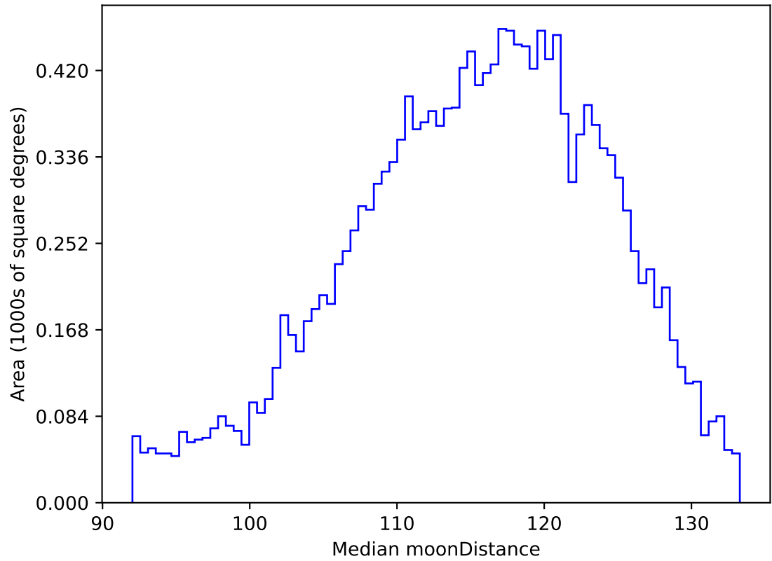
roll_uniform_early_half_mjdp0_v3.4_10yrs WFD g band: Median moonDistance
