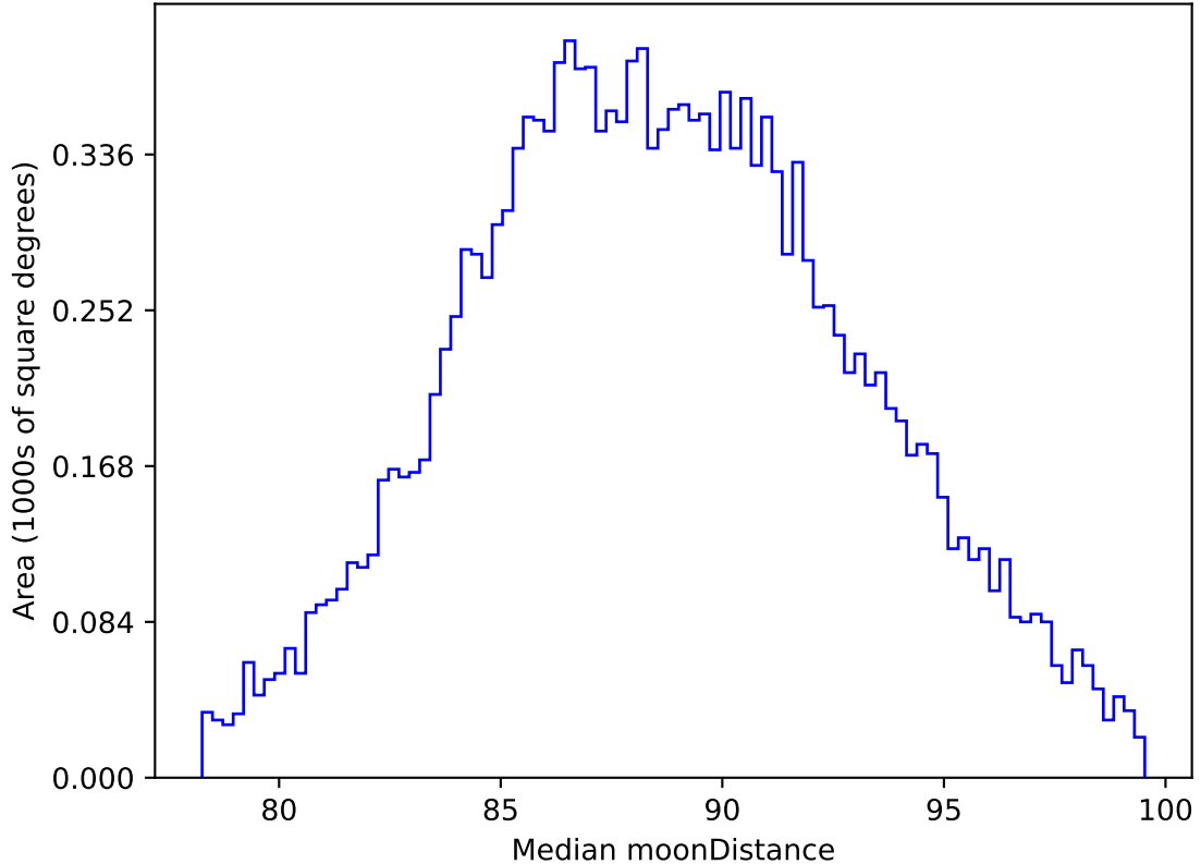
roll_uniform_early_half_mjdp0_v3.4_10yrs WFD all bands: Median moonDistance
