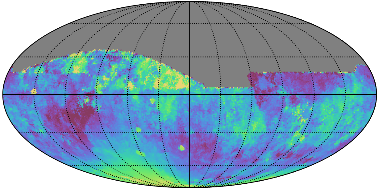
roll_uniform_early_half_mjdp0_v3.4_10yrs All sky z band: Median moonDistance
