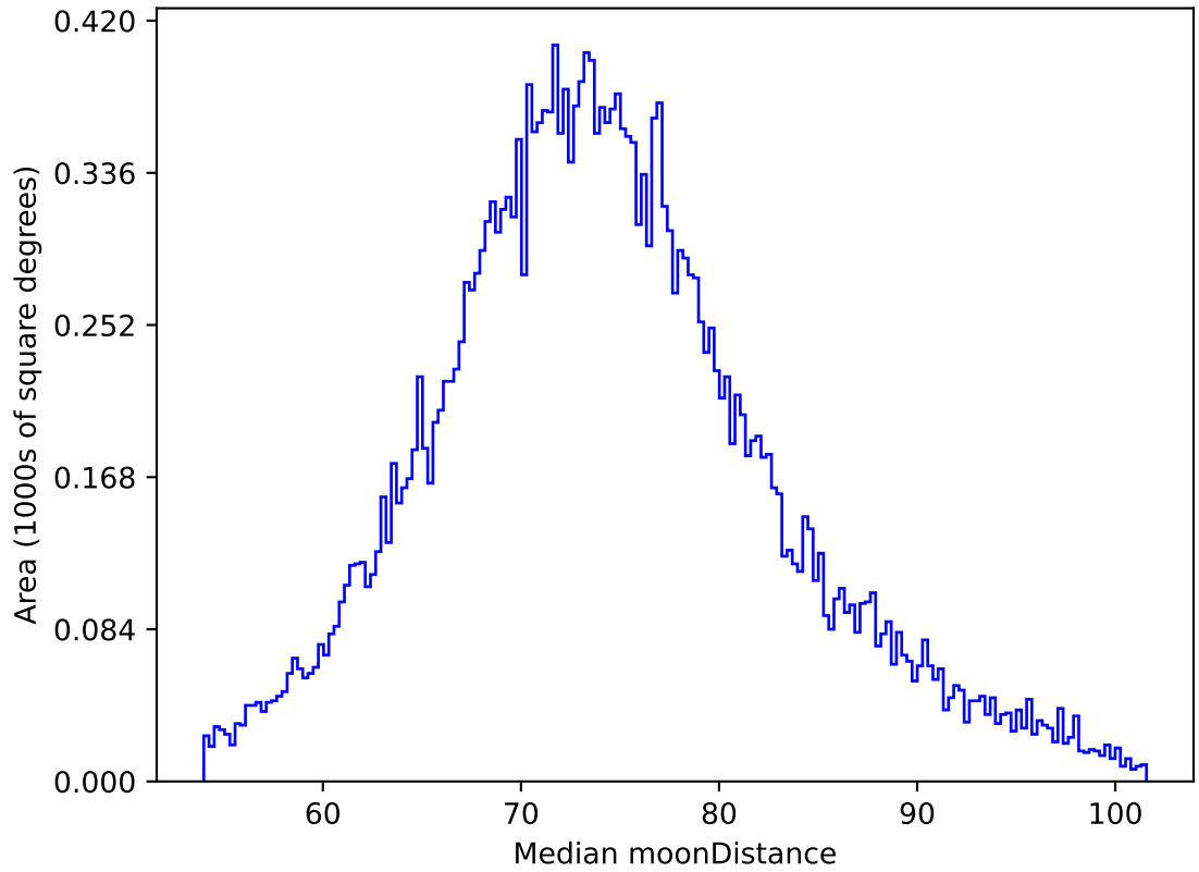
roll_uniform_early_half_mjdp0_v3.4_10yrs All sky z band: Median moonDistance
