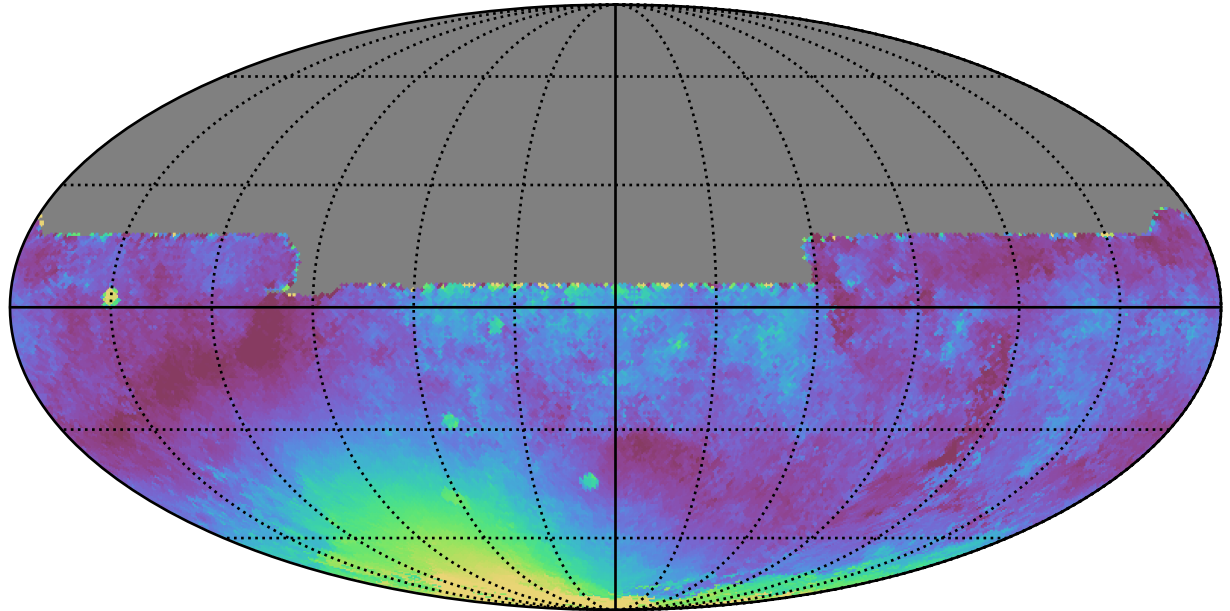
roll_uniform_early_half_mjdp0_v3.4_10yrs All sky y band: Median moonDistance
