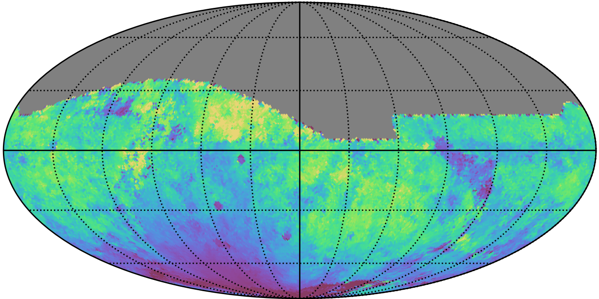
roll_uniform_early_half_mjdp0_v3.4_10yrs All sky r band: Median moonDistance
