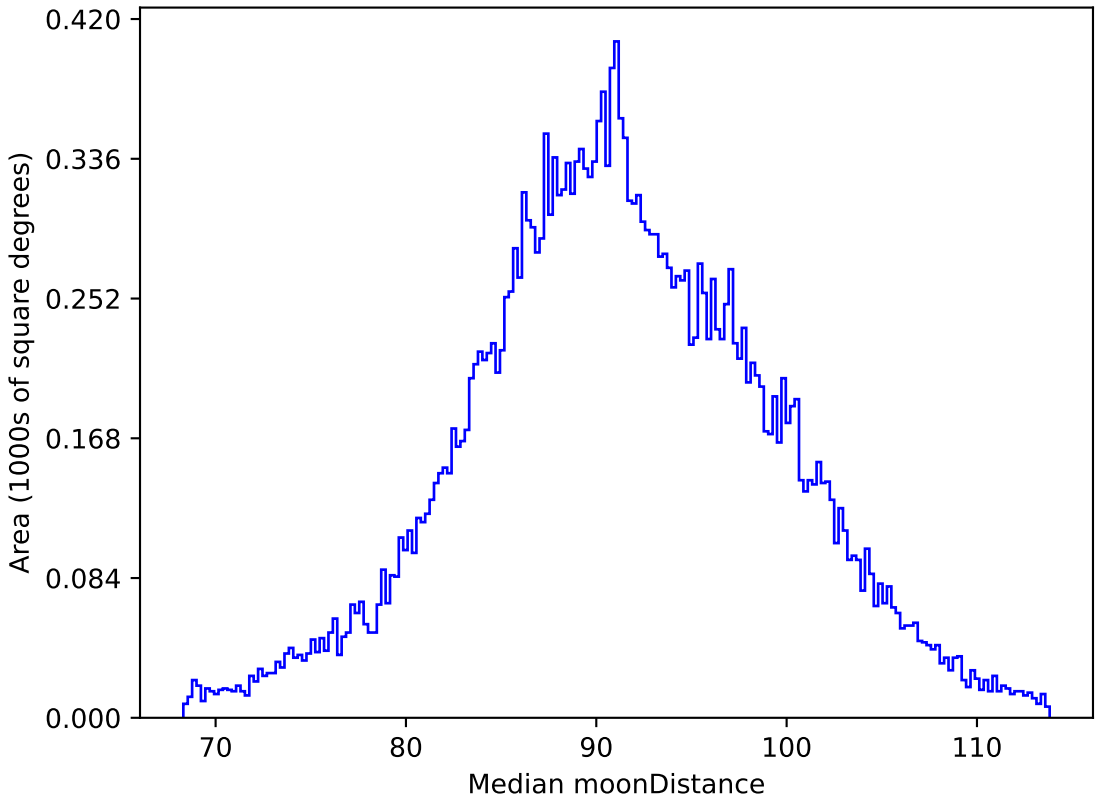
roll_uniform_early_half_mjdp0_v3.4_10yrs All sky i band: Median moonDistance
