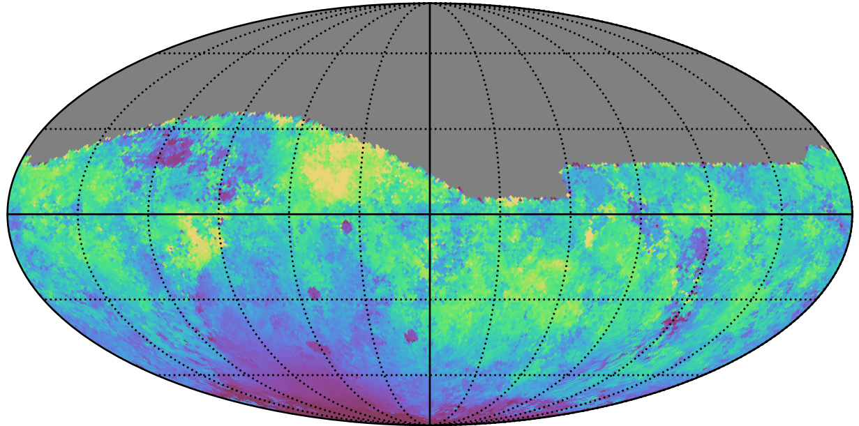
roll_uniform_early_half_mjdp0_v3.4_10yrs All sky g band: Median moonDistance
