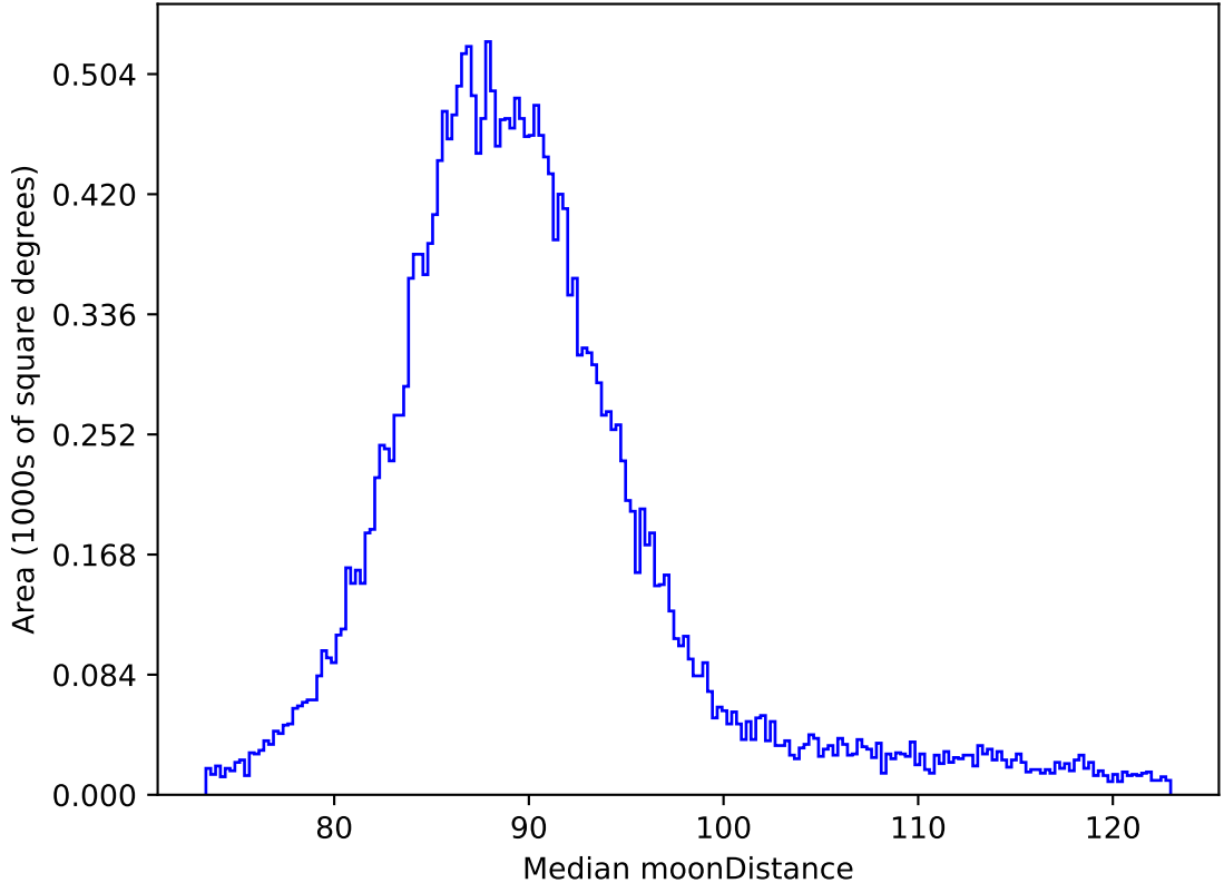
roll_uniform_early_half_mjdp0_v3.4_10yrs All sky all bands: Median moonDistance
