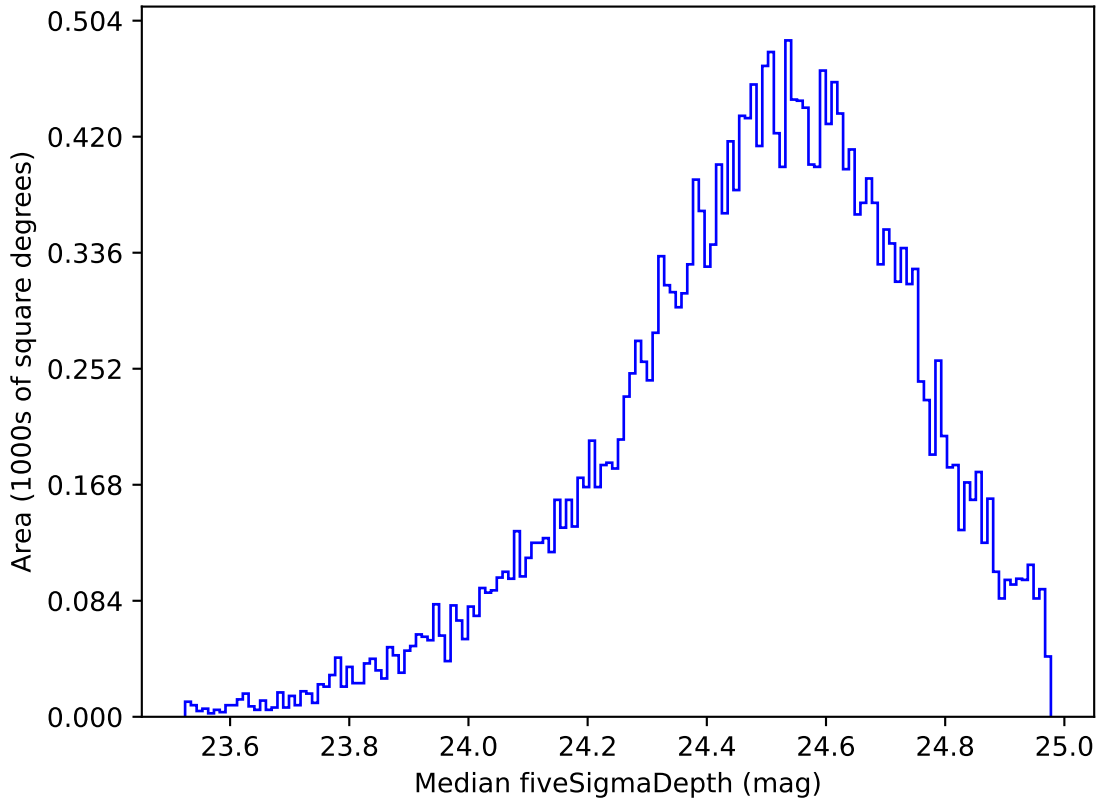
roll_uniform_early_half_mjdp0_v3.4_10yrs Yr 1 g band: Median fiveSigmaDepth
