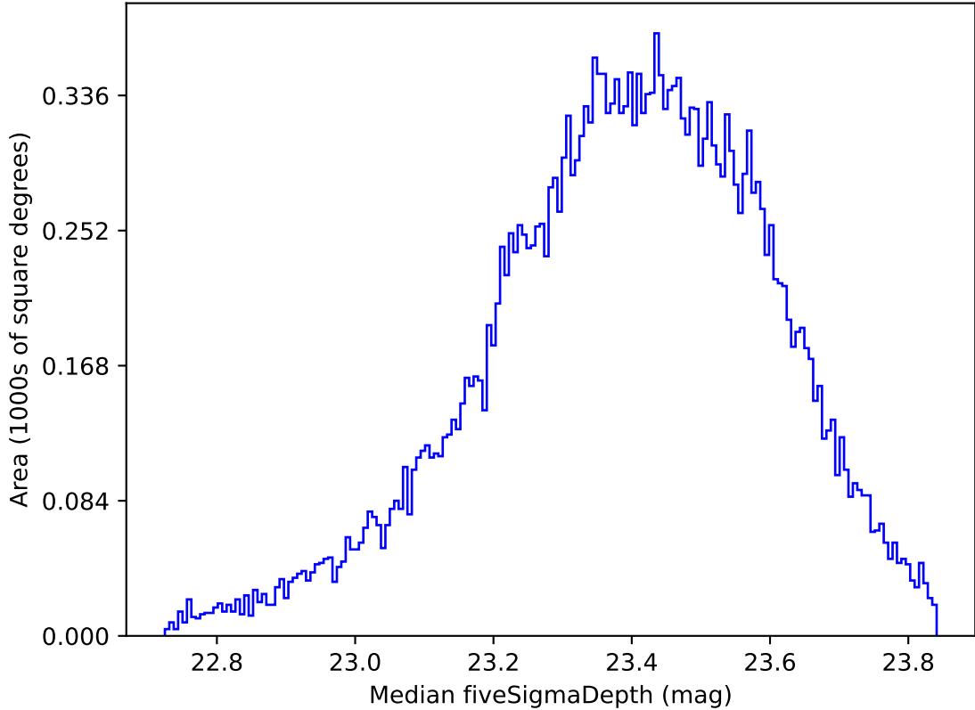
roll_uniform_early_half_mjdp0_v3.4_10yrs Yr 1 all bands: Median fiveSigmaDepth
